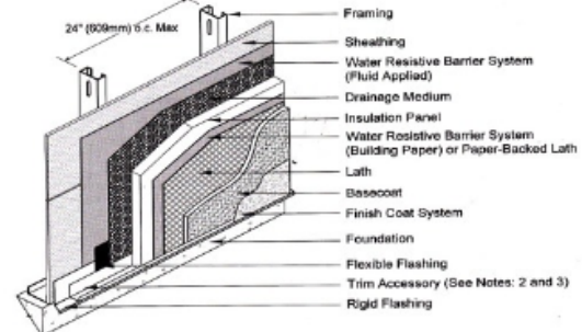
Stucco Continuous Insulation Rainscreen System
