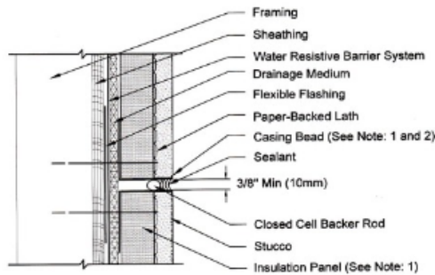
Stucco Horizontal Control Joint
