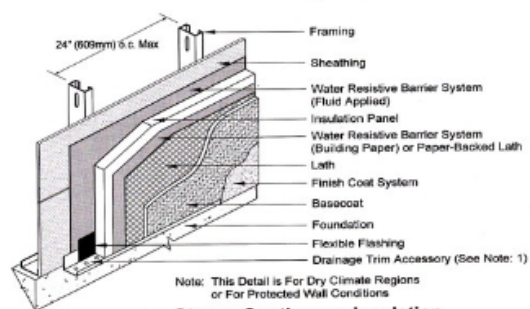
Stucco Continuous Insulation
